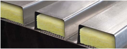
Type "N-Cellular" Acoustical Type Shown
