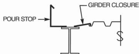
TYPICAL POUR STOP AND GIRDER CLOSURE APPLICATION
