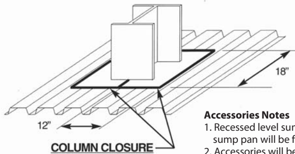
COLUMN CLOSURE
