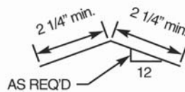
RIDGE AND VALLEY PLATE (20 GAGE MIN.)
