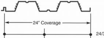
3" Composite
