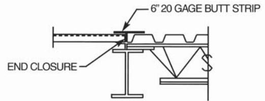
DETAIL WHERE DECK CHANGES DIRECTION
