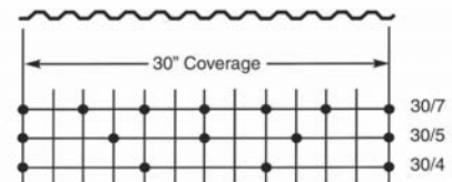
9/16", Type "S"
