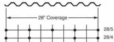
7/8", Type "HD"
