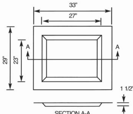
SECTION A-A RECESSED SUMP PAN LEVEL (14 GAGE MIN.) (HOLE CUT IN FIELD BY OTHERS)
